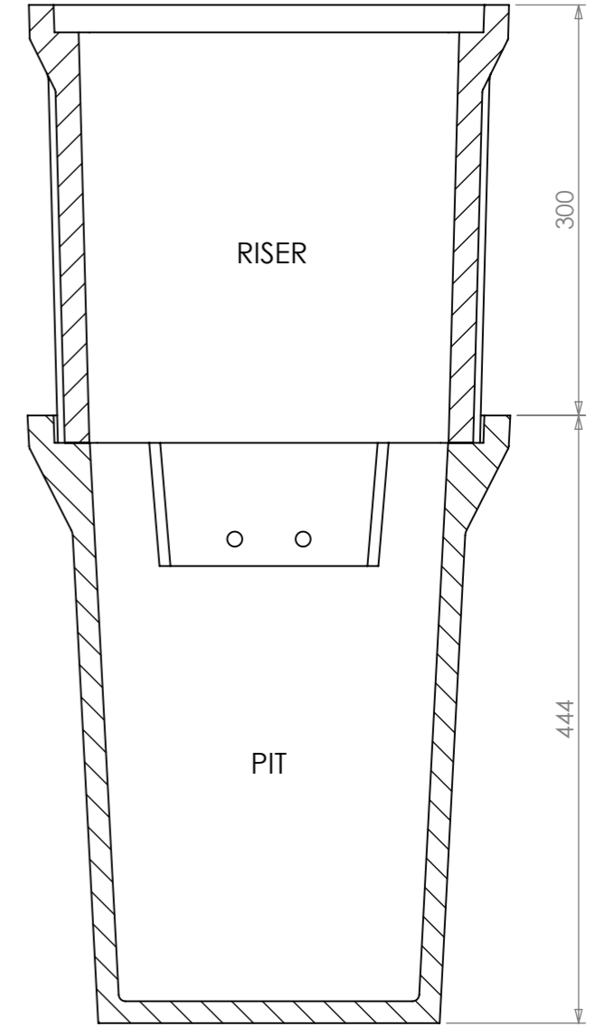
PIT & RISER ASSEMBLY
