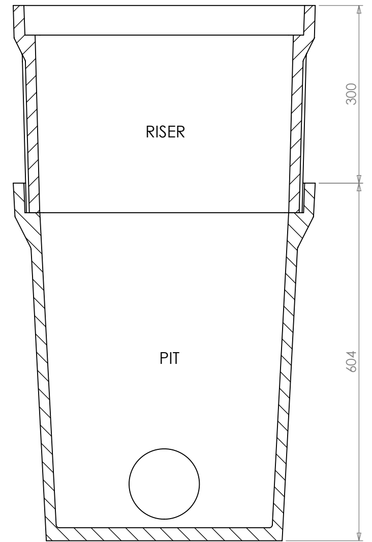
PIT & RISER ASSEMBLY
