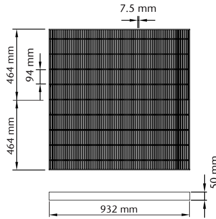
Galvanised Heelguard 2 - Part grate
