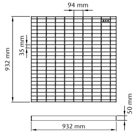
Galvanised Transverse grate
